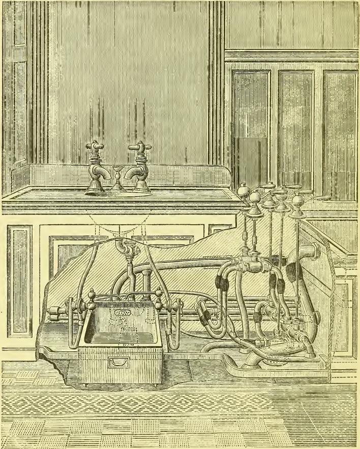
FIG. 14.—Plumbing in a bath-room in the house of Governor S. J. Tilden. ("Sanitary Engineer.")
